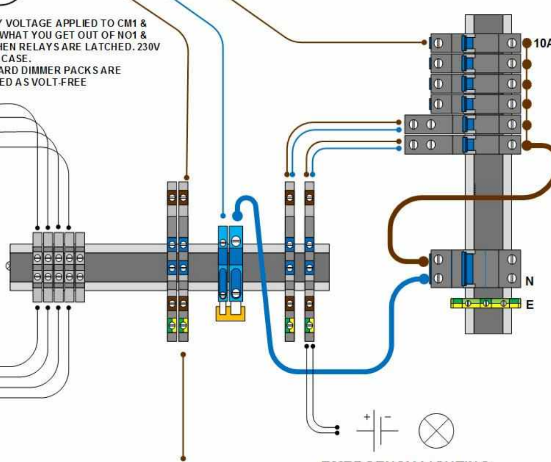
EMERGENCY LIGHTING CIRCUIT 230V
